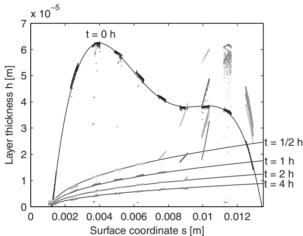
Figure 10.5 Solution of Eq. 10.3 and measurements for the layer thickness on a raceway of a tapered roller bearing inner-ring ( L = 13.5 mm; R = 25.4 mm; \alpha = 10.9^\circ , \nu = 1370 cSt ( 1.25 \text{ Pa} \cdot \text{s} )). The drawn lines are the model calculations and the dots denote measured values. Reproduced from van Zoelen et al. , 2008 © ASME.
